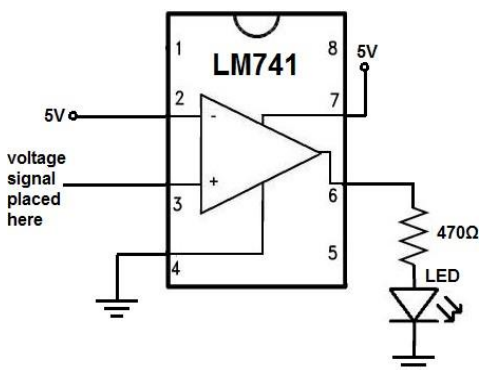
Voltage Sensor
