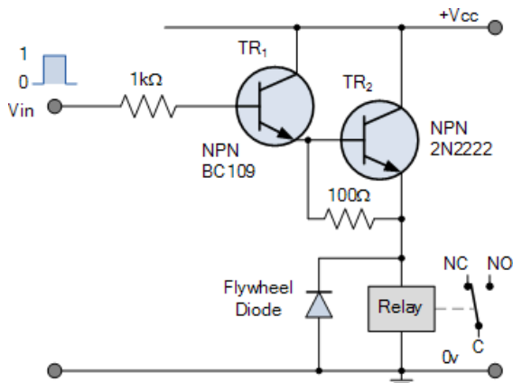
Relay Circuite
