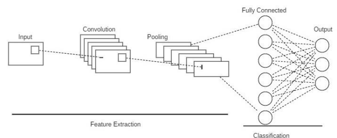
Fig 2-Convolutional Neural Network
