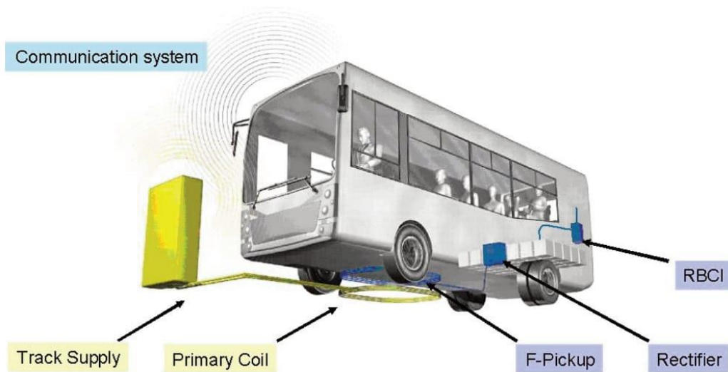
Figure 1. Major Components for Typical 30-kW Inductive Charge System, Block Diagram
