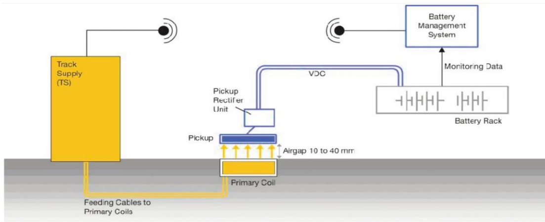
Figure 1. Major Components for Typical 30-kW Inductive Charge System, Block Diagram
